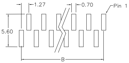
P.C. Board Layout Type A
