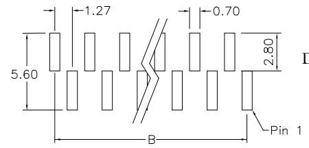
P.C. Board Layout Type B
