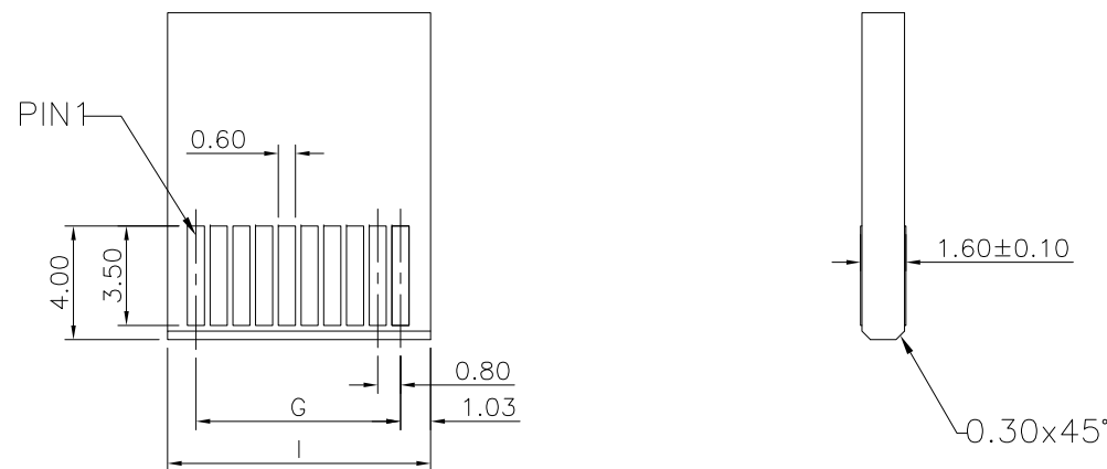
RECOMMENDED MATTING BOARD FOOTPRINT (Tolerance: \pm 0.05 )
