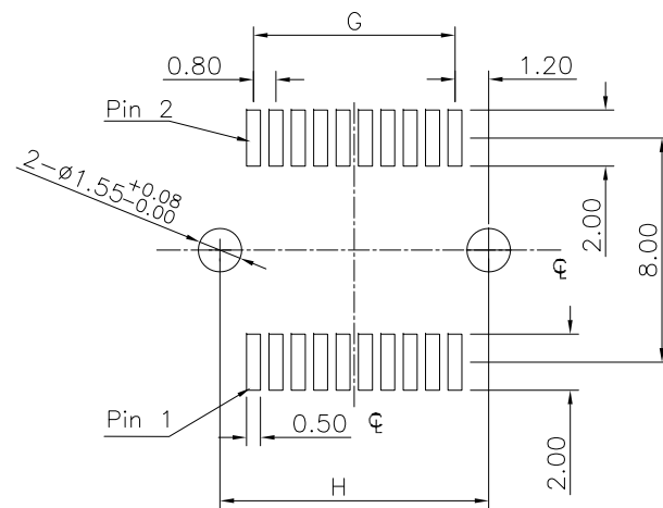
P.C. Board Layout (Tolerance \pm 0.05 )
