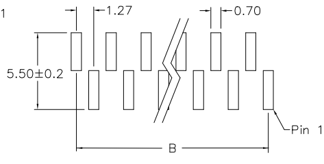
P.C. Board Layout Type B
