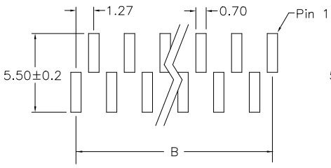
P.C. Board Layout Type A
