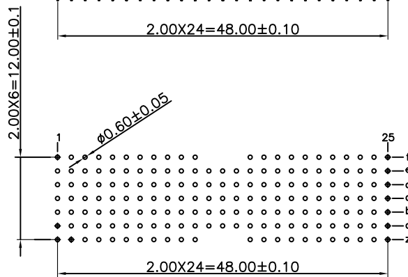
P.C. Board Layout (Top View)
