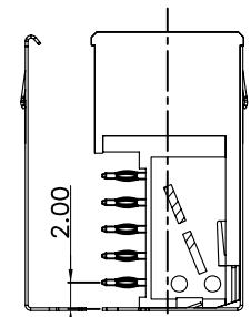
With Top Body Shielded and Bottom Shielded
