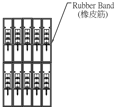
Drawing Two: Each Bundle Ten Tube (圖二: 每10管為1捆)
