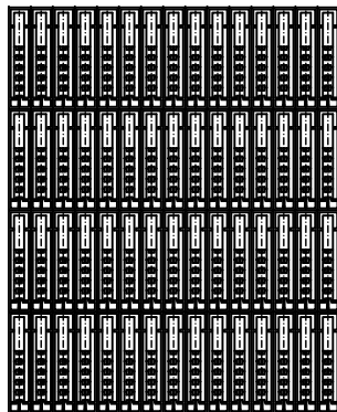
Drawing Three:Lay three bundles in each layer.Install in two layers.Six bundles, Sixty tubes in all.
