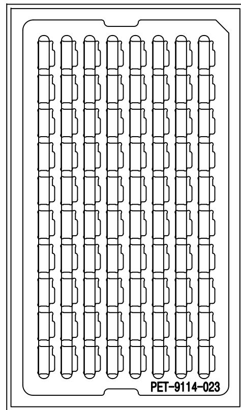
(Drawing 1-1) (圖1-1)
