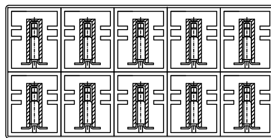
Drawing Two: Each Bundle 10 Tube (圖二: 每10管為1捆)
