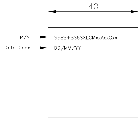
LABEL DETAIL
