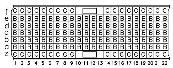
CONTACT LAYOUT
