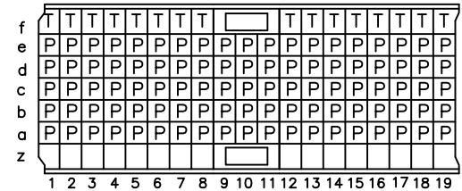
CONTACT LAYOUT
