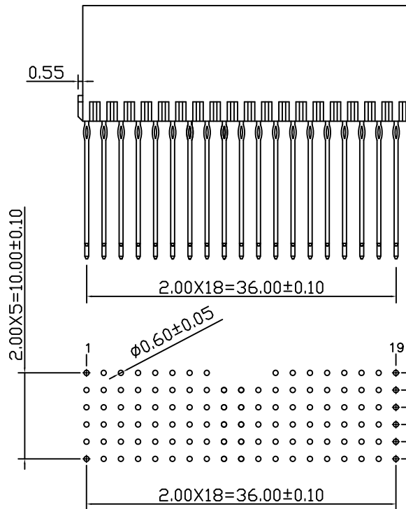
P.C. Board Layout (Top View)
