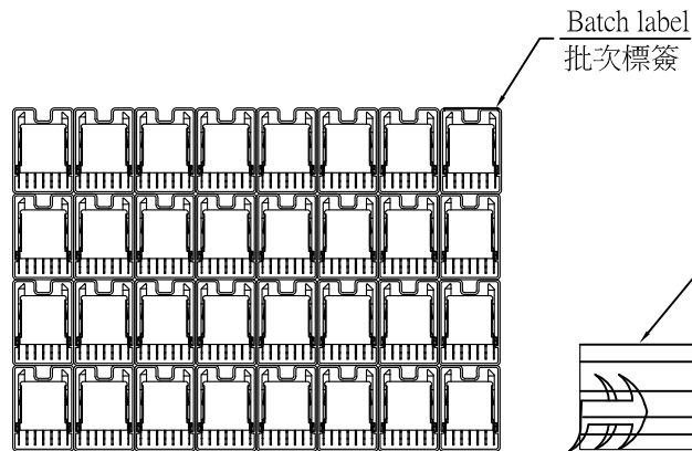
(圖三) Drawing Three: Lay two bundle in each layer. Install in 4 layers. 8 bundles, 32 tubes in all. (圖3)每層放2捆。分4層放入,一盒共8捆,共32管 Disposing schematic diagram of Tube in the inner box, for reference. (管在內盒的擺放示意圖,供參考)
