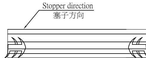
(圖三) Drawing Three: Lay two bundle in each layer. Install in 4 layers. 8 bundles, 32 tubes in all. (圖3)每層放2捆。分4層放入,一盒共8捆,共32管 Disposing schematic diagram of Tube in the inner box, for reference. (管在內盒的擺放示意圖,供參考)
