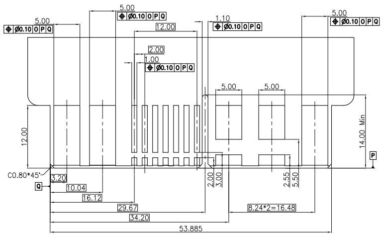
RECOMMENDED MATTING BOARD FOOTPRINT (Tolerance:±0.05)
