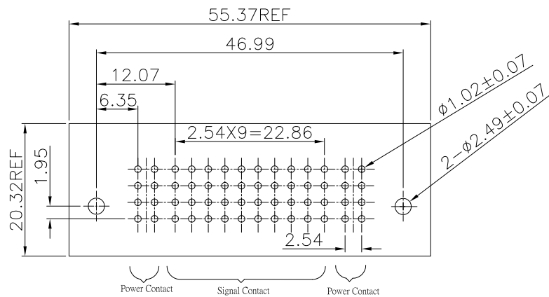
P.C.Board Layout (Tolerance:±0.05)
