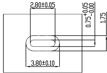
P.C. Board Layout (Tolerance=0.05mm) THICKNESS:2.50mm Min
