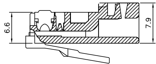
Section A-A' (8 & 10 Position)
