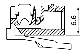
Section A-A' (4 & 6 Position)
