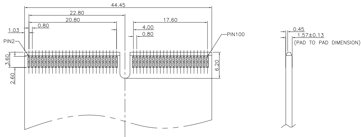
RECOMMENDED MATTING BOARD FOOTPRINT (Tolerance \pm 0.05 )
