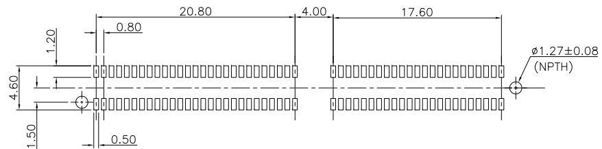
P.C. Board Layout (Tolerance \pm 0.05 )
